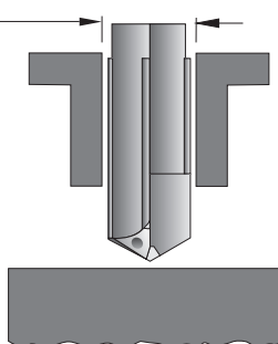
Bushing away
