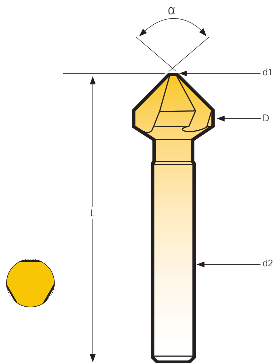
Countersink
