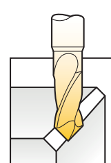
90°-120° Centering - Spotting
