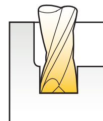
Slotting Engraving
