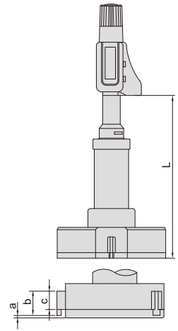
Type C 2-12", carbide points
