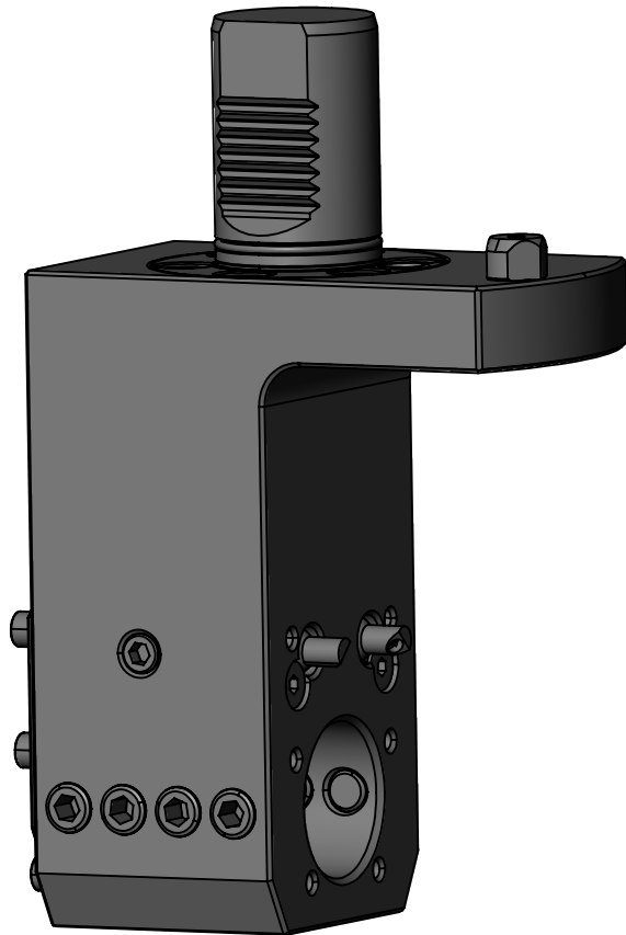
90 DEGREE VDI40 STATIC TOOL OUTPUT: 1.1/2" BORING BAR COOLANT: EXTERNAL & INTERNAL **BACK PLATE REMOVABLE**
