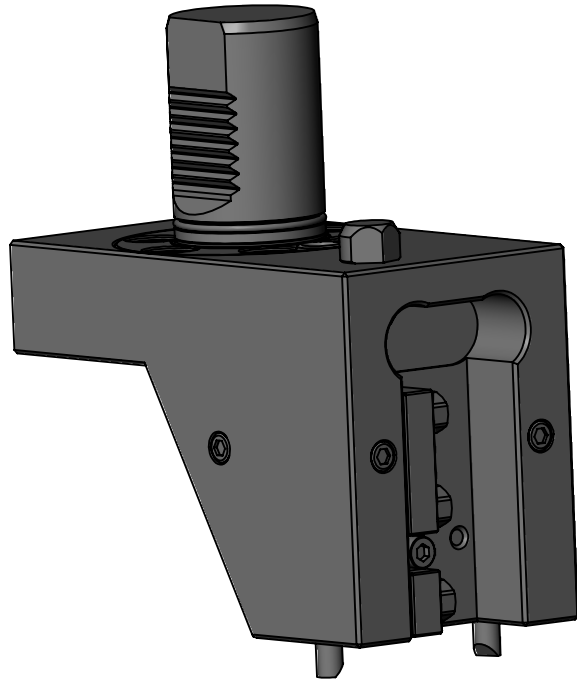
STRAIGHT VDI40 STATIC TOOL OUTPUT: 3/4" SQR SHANK COOLANT: EXTERNAL **WEDGE CLAMP MOVABLE LEFT/RIGHT**
