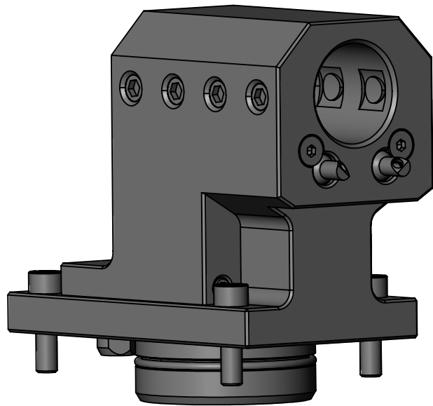
90 DEGREE STATIC TOOL OUTPUT: 1.1/2" BORING BAR MAIN & SUB COOLANT: EXTERNAL
