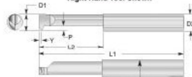
Lockdown flat automatically locates tool on center
