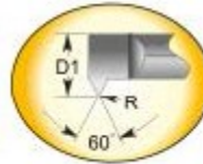
Tool Radius: .002" ±.001"
